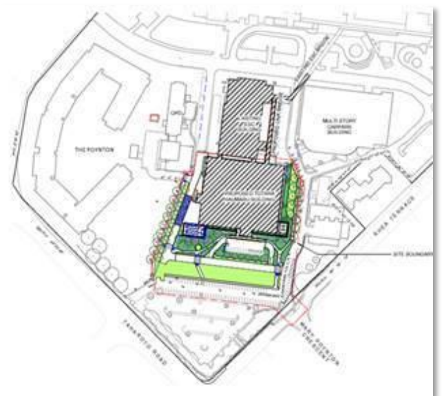
Site drawing of the new hospital and grounds
